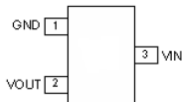
SOT23-3L(Top View)
