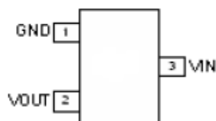
SC70-3L(Top View)
