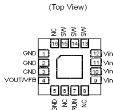
QFN3*3-16L
