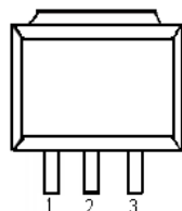
2) TO252-3L (Top View)
